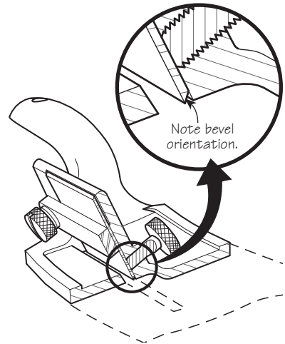
Figure 5: Set-up.
