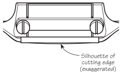
Figure 6: Adjustment.
