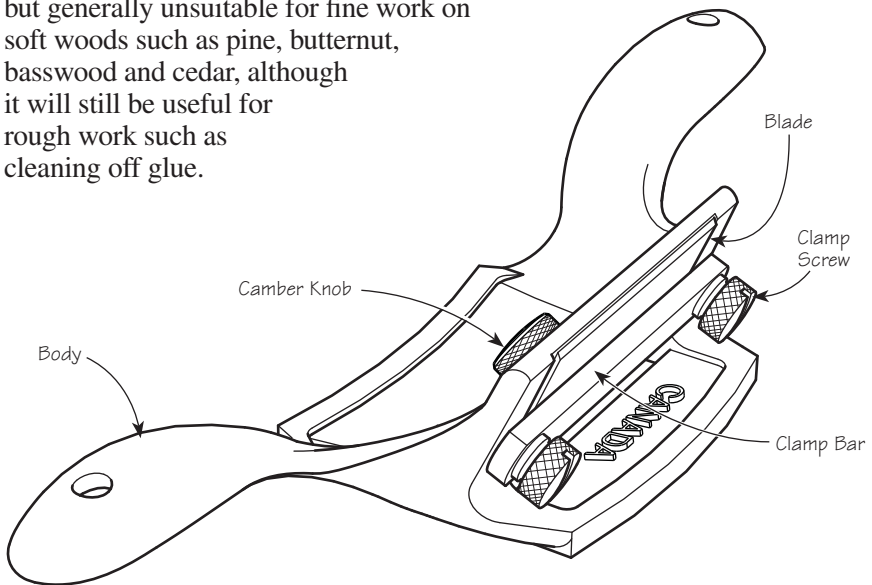
Figure 1: Cabinet scraper components.
